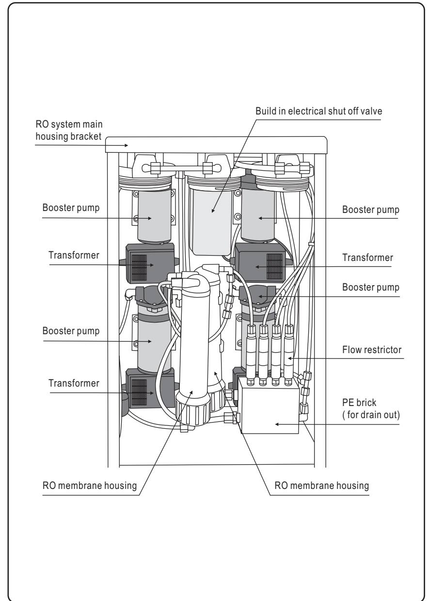
RO800 800GPD Light Commercial
